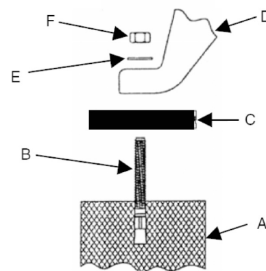
Typical Mounting
